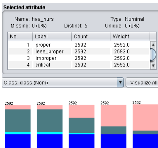
Slika 16. dio 'Selected attributes' u prozoru 'preprocess'
