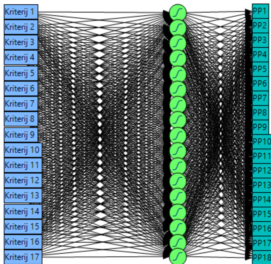
Figure 1: The structure of the neural network in the case of the City of Zabok
