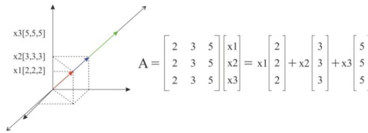
Figure 1: Matrix A rank 1
