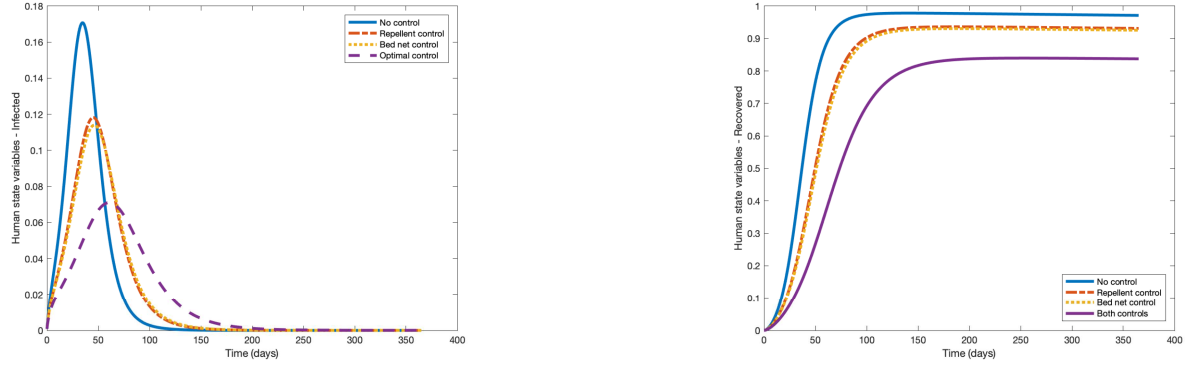
Figure 1: State variables, infected ( i ) and recovered ( r ), for the multiple strategies
