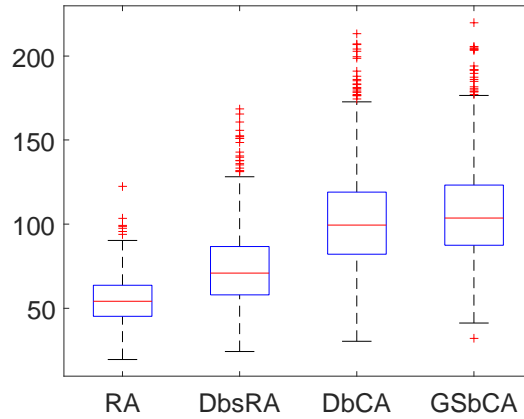
Figure 1: Total capacity in MBps in the case of the various assignment algorithms. In the box plot, the central mark is the median, while the edges of the box are the 25th and 75th percentiles respectively. The whiskers extend to the most extreme data points which are considered not to be outliers, and the outliers are plotted individually with red crosses. The median values are respectively 54.18, 70.87, 99.38 and 103.63 for the four algorithms.
