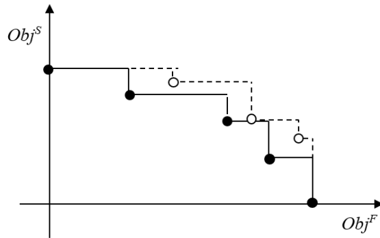
Figure 2: The black circled correspond to the Pareto front members and the empty circles denote the members of the approximation
