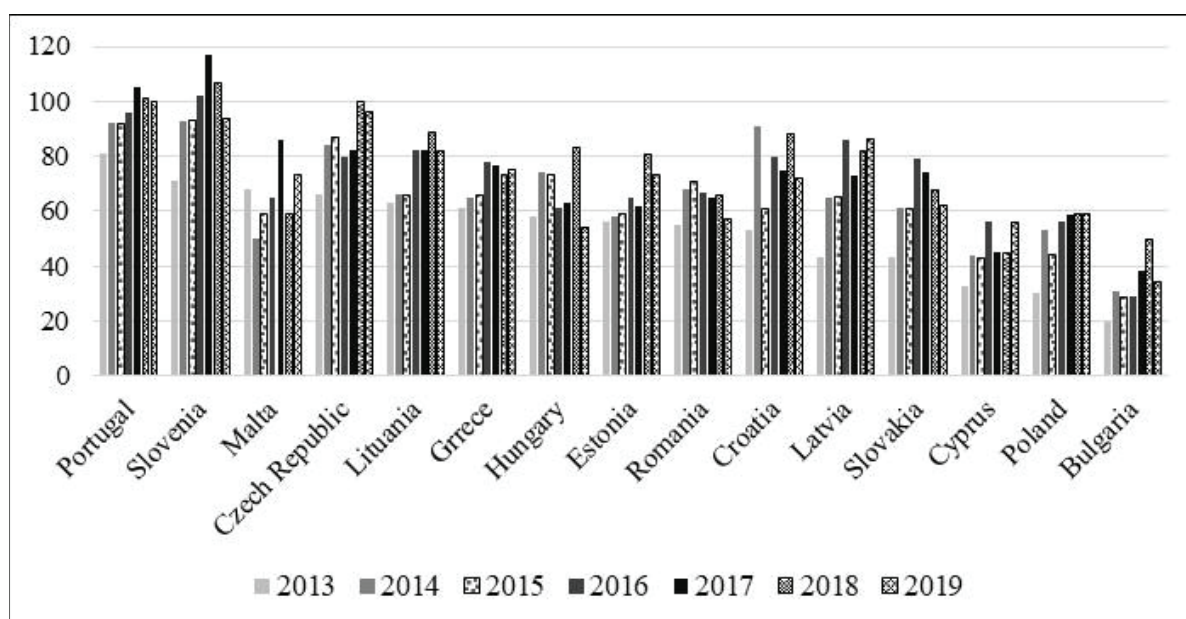
Figure 2: Eco-II catching-up countries 2013-2019
